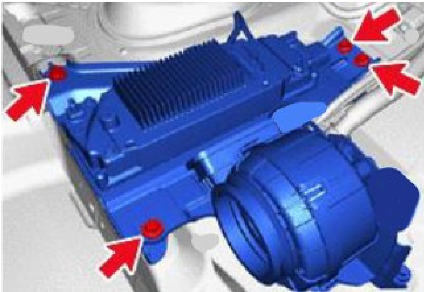
DC/DC transformers/converters
