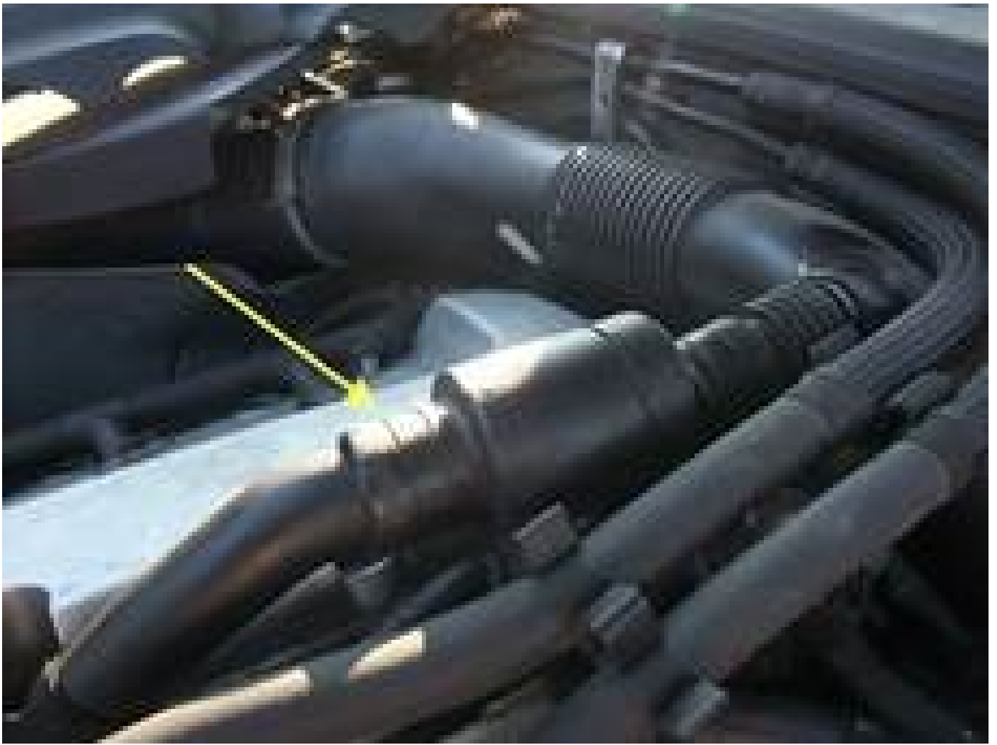
Figure 3: View / location in the engine compartment with cover
