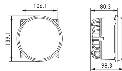
Dimensional sketches of the Bi-LED low beam and high beam headlamp M133 LED (R149 Class DS)
