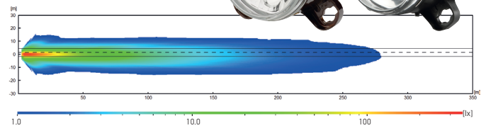
Halogen Performance (247 043 + 247 042)
