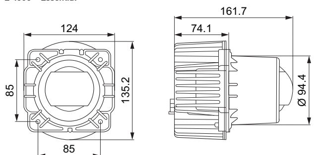
Dimensional sketches of the Bi-LED low beam and high beam headlamp L 4565 - Essential
