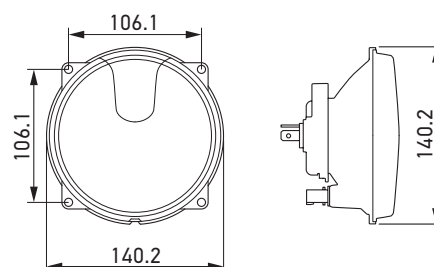
Dimensional sketches of the Bi-halogen low beam and high beam headlamp M133 (R149 Class DS)
