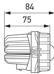
Dimensional sketches of the LED low beam headlamp Module 60 LED
