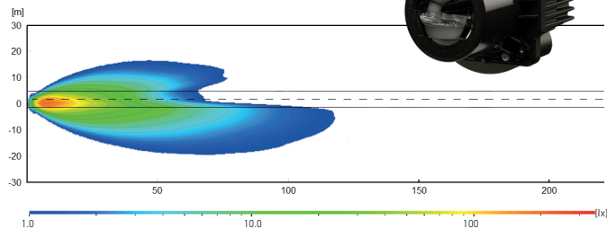
Bi-LED Essential L 4565 (015 318)
