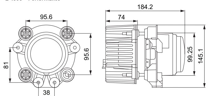
Dimensional sketches of the Bi-LED low beam and high beam headlamp L 4565 – Performance
