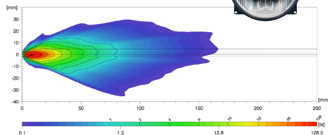
M133 LED (R149 Class DS) (996 362)
