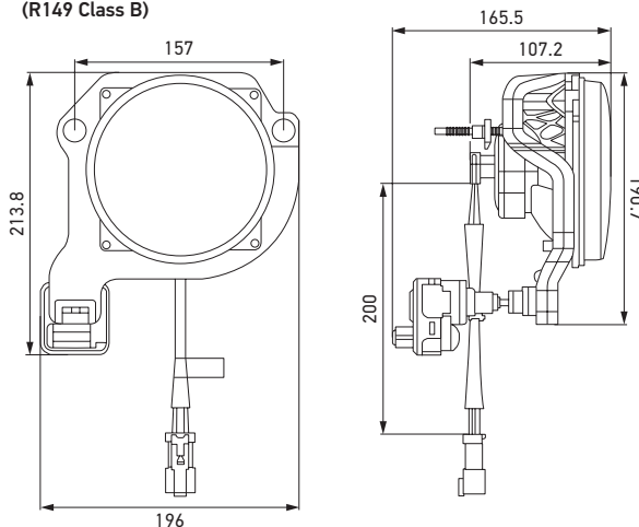
Dimensional sketches of the Bi-halogen low beam and high beam headlamp M133 (R149 Class B)
