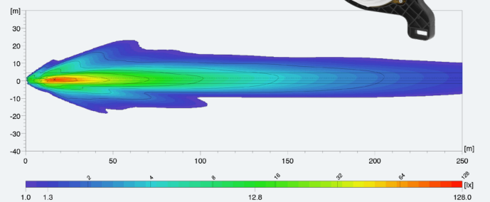
M133 Halogen (R149 Class B) (997 262)
