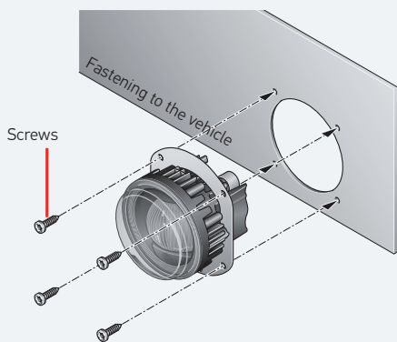
Installation example 2 With pre-assembled carrier frame
