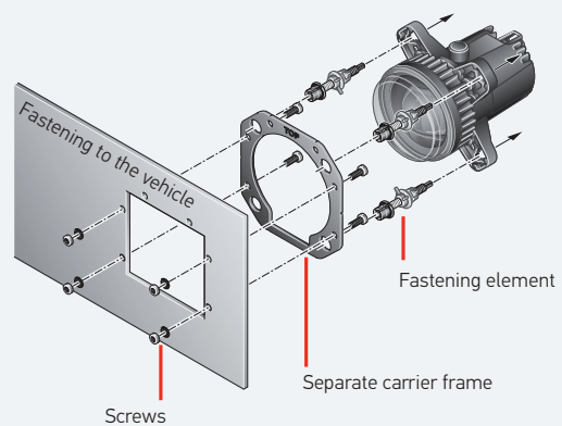
Installation example 3 With additional carrier frame
