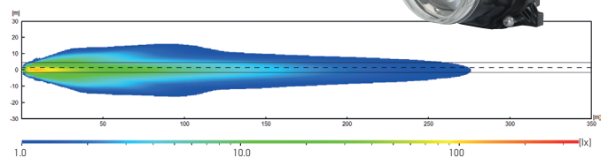
Bi-halogen Performance (009 998)
