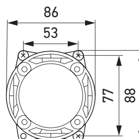
With carrier frame, vertical (Horizontal mounting also possible)
