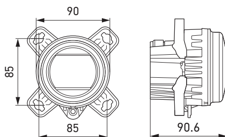
Without carrier frame
