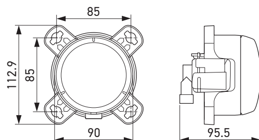
Dimensional sketches of the halogen high beam headlamp
