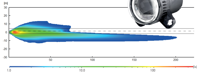
LED Performance L 4060 (012 488)
