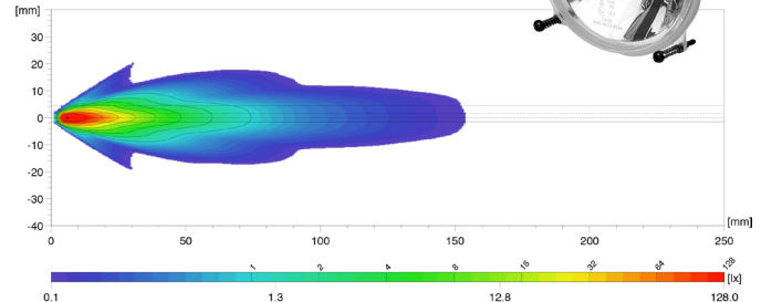
M133 Halogen (R149 Class DS) (996 262)
